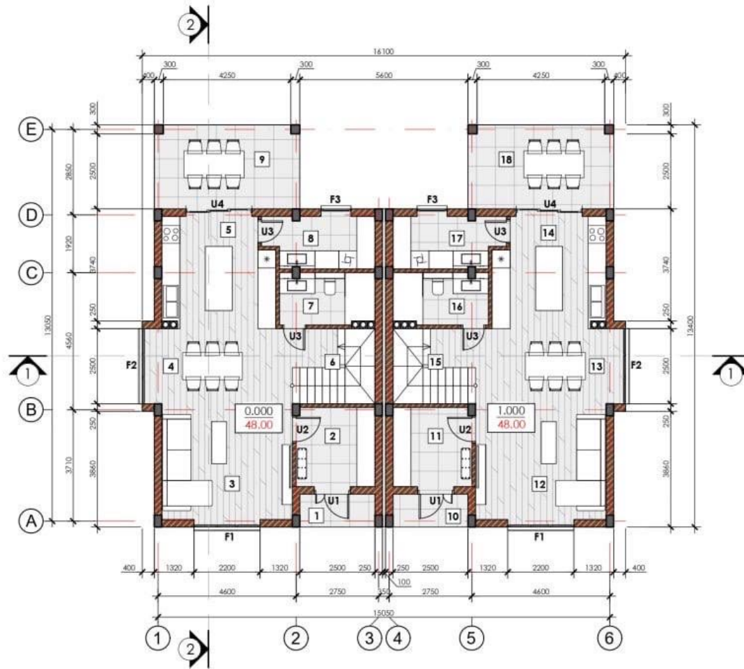
Plan parter, sc. 1:100, amplasare mobilier
